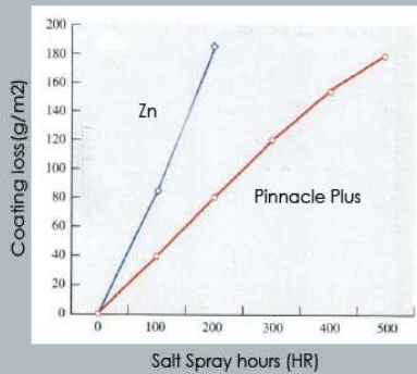
Salt spray test result for 1mm wire
