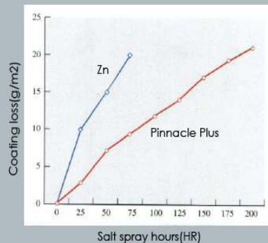
Salt spray test result for 5mm automotive cable
